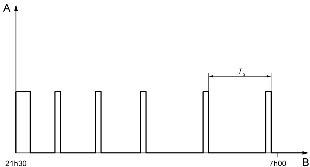
Figure A.4 — Load profile - Test cycle for measurement of the energy consumption of the appliance without storage tank maintained in temperature
